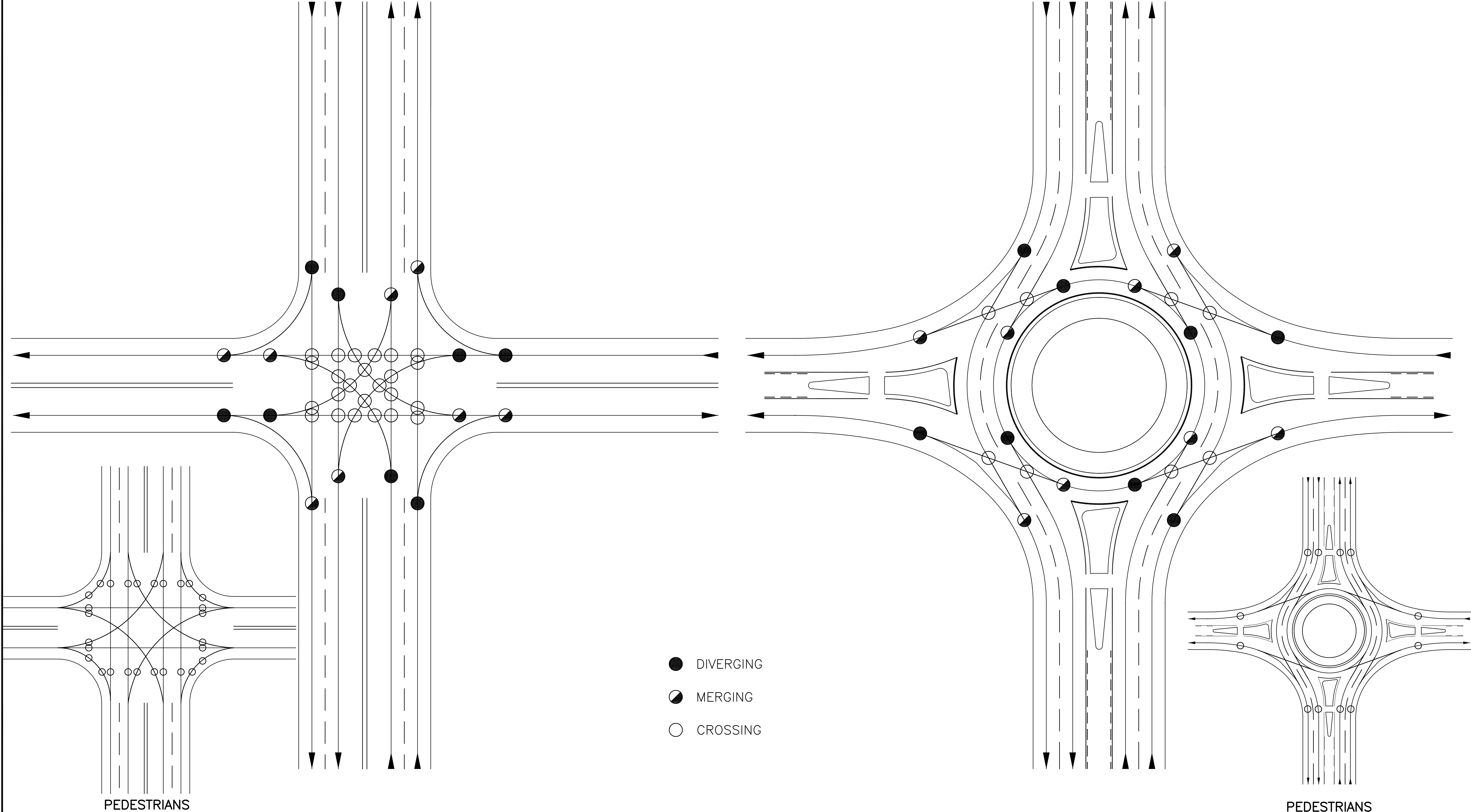
TRADITIONAL INTERSECTION
