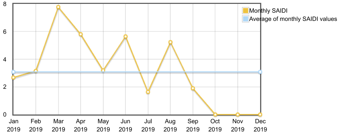
Monthly SAIDI Chart
