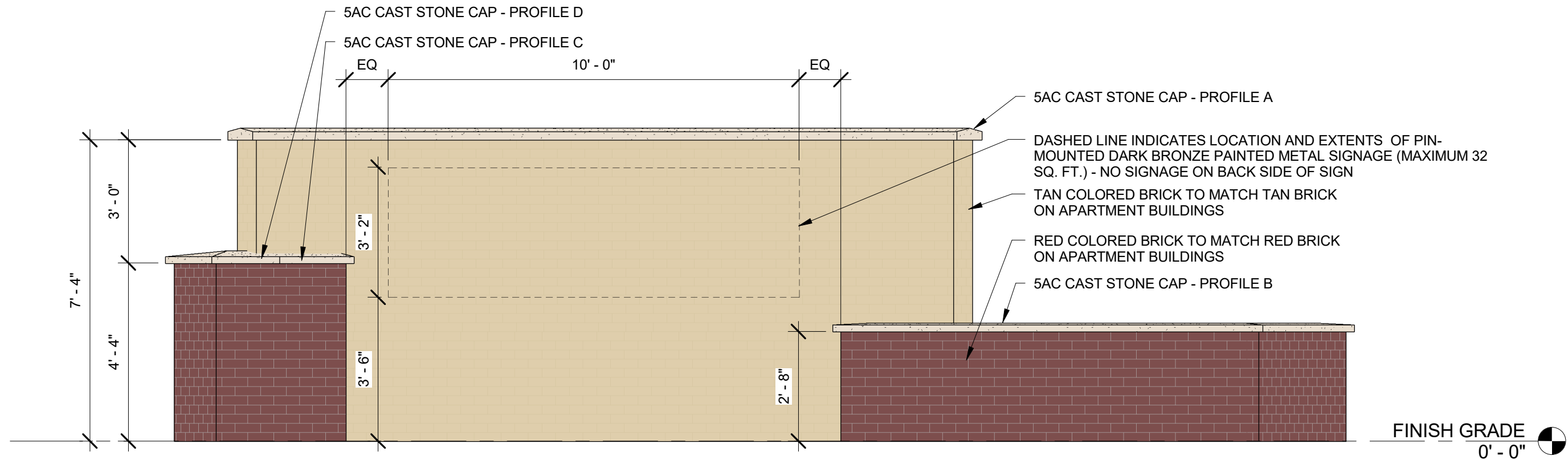
① ELEVATION FACING ROUNDABOUT (OPP. SIDE SIMILAR) 3/8" = 1'-0"
