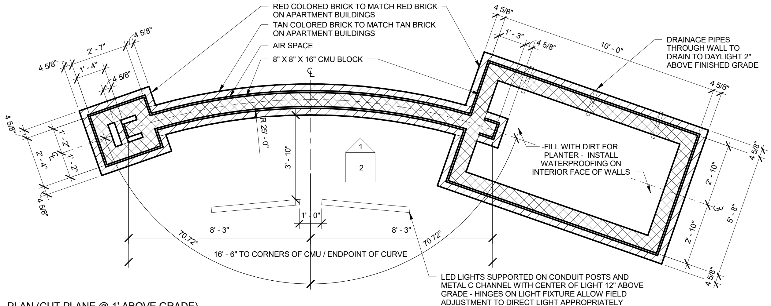
① PLAN (CUT PLANE @ 1' ABOVE GRADE) 3/8" = 1'-0"
