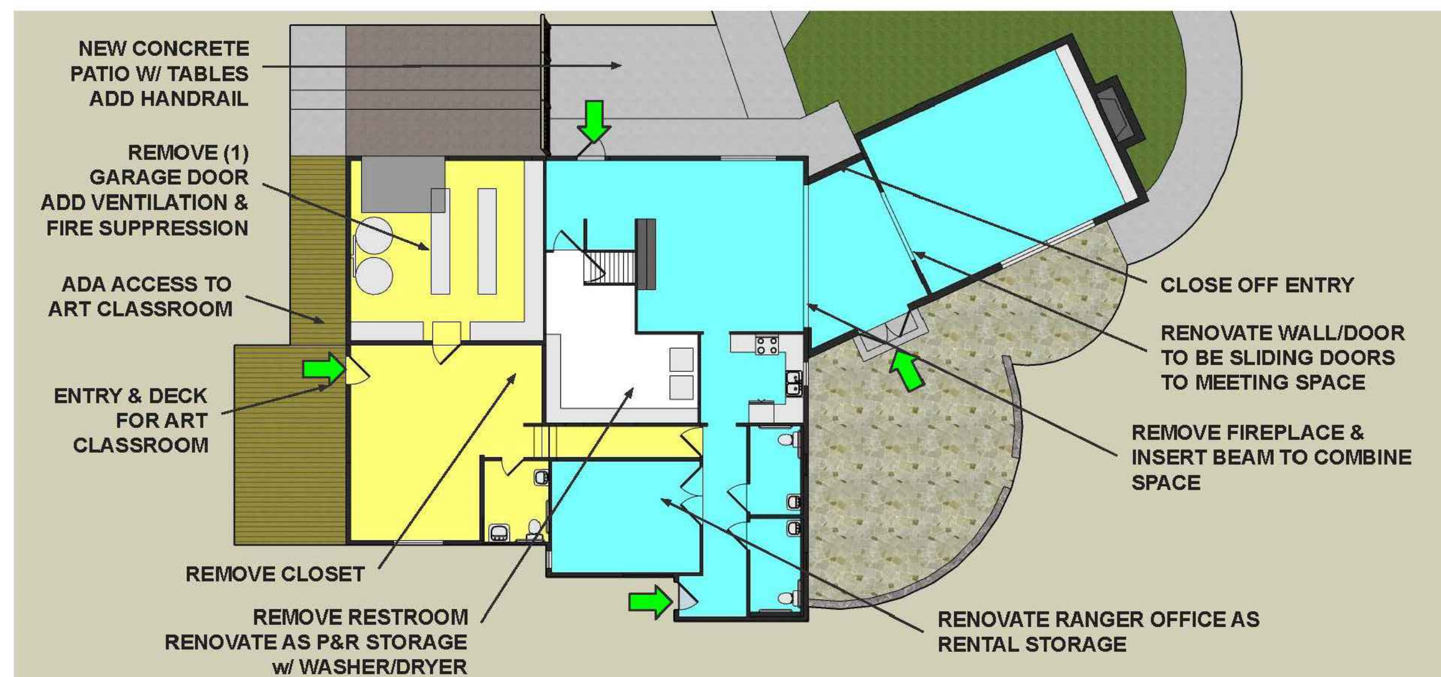
WATERS HOUSE - PROPOSED IMPROVEMENTS A
