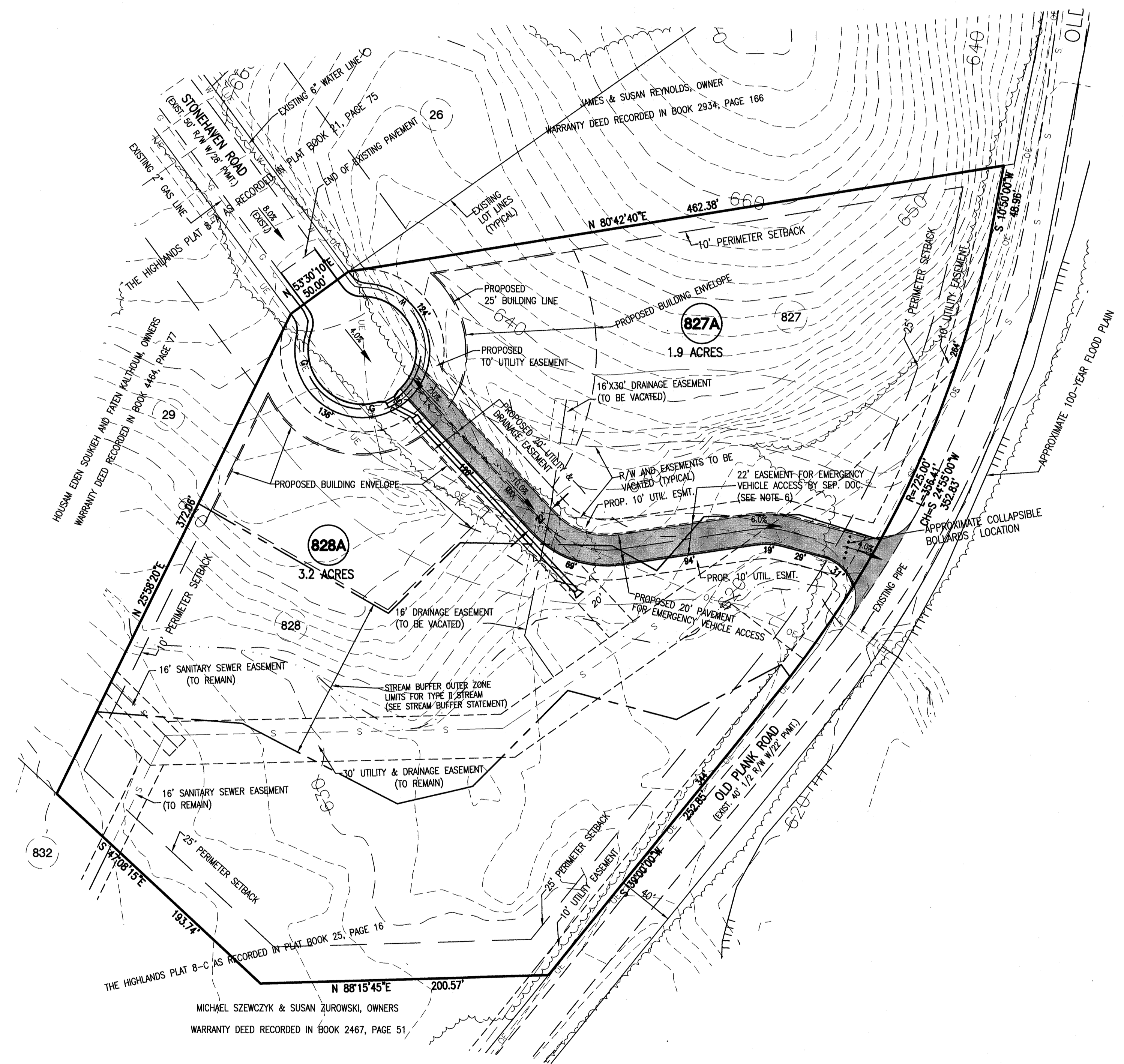
TYPICAL LOT LAYOUT (NOT TO SCALE)
