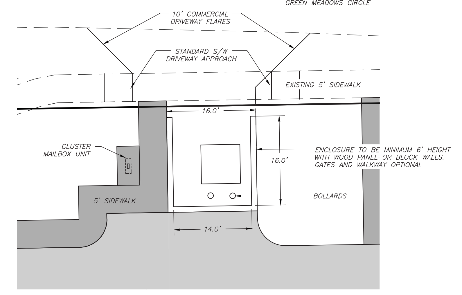
TRASH ENCLOSURE & MAILBOX DETAIL
