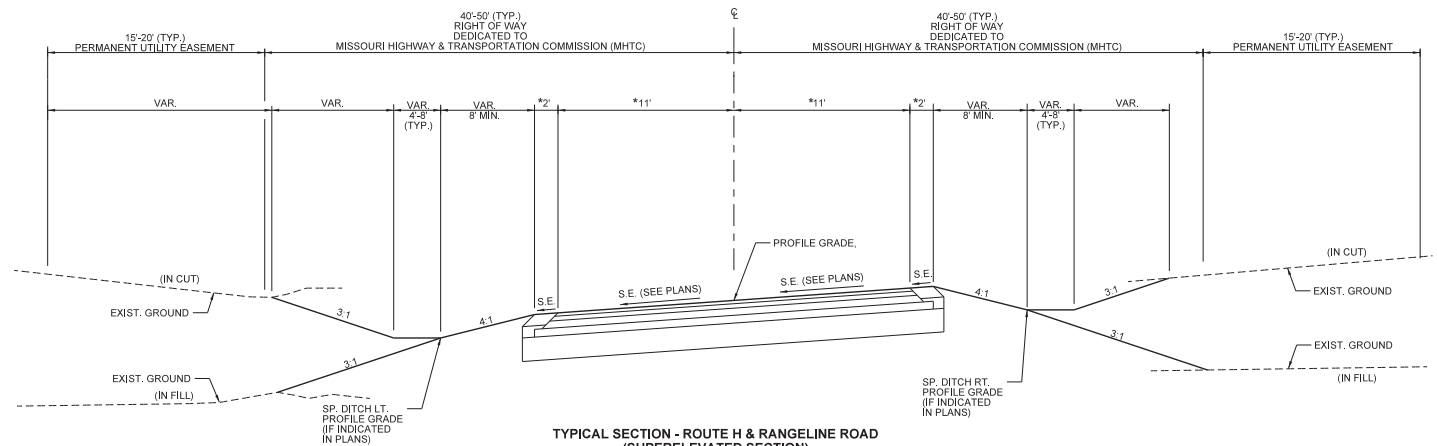
TYPICAL SECTION - ROUTE H & RANGELINE ROAD (SUPERELEVATED SECTION) (TYPICAL IS FOR CURVE TO THE LEFT - MIRROR PAVEMENT FOR CURVE TO THE RIGHT) (FOR INFORMATION ONLY)
