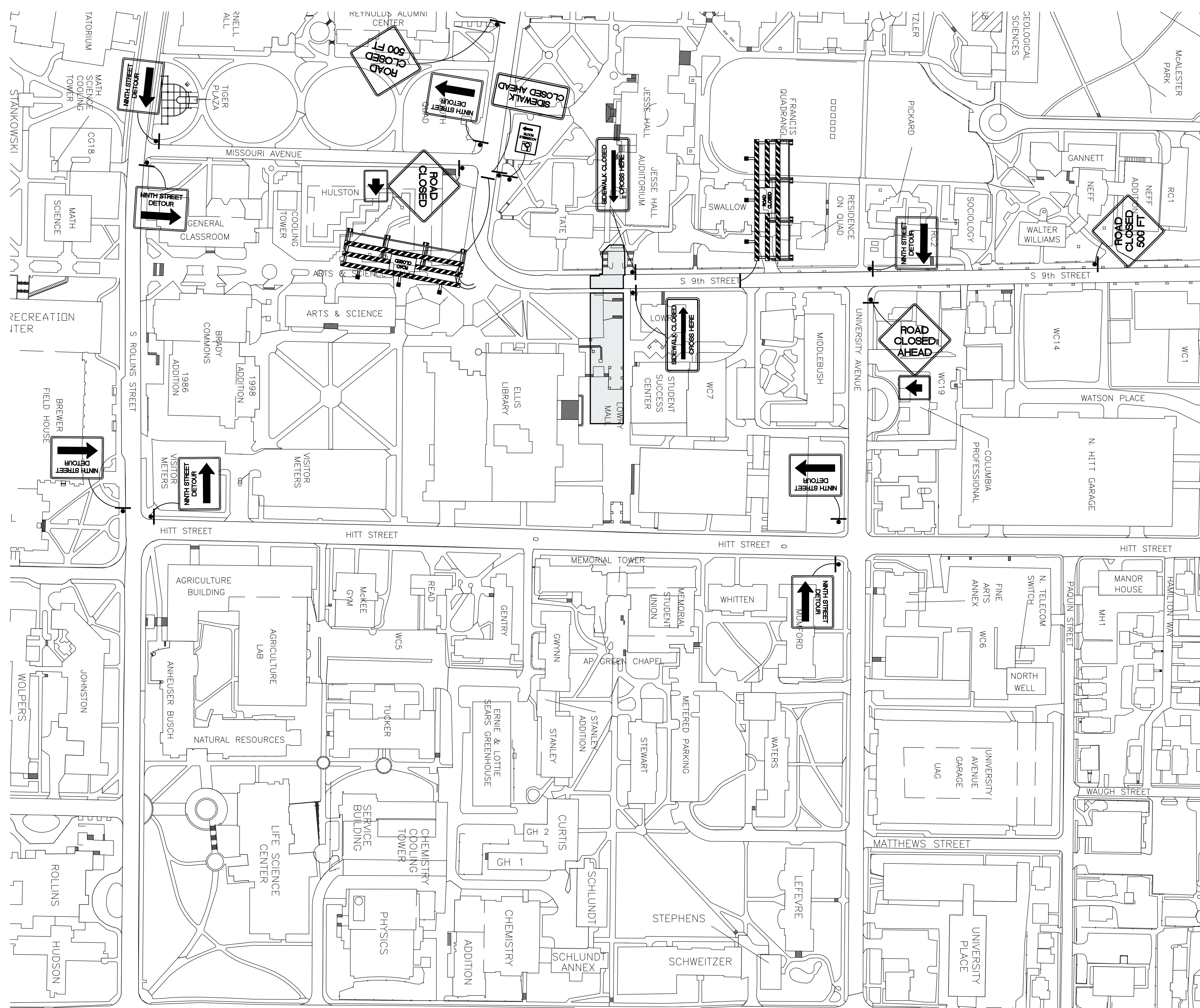
PHASE 2 TRAFFIC CONTROL PLAN
