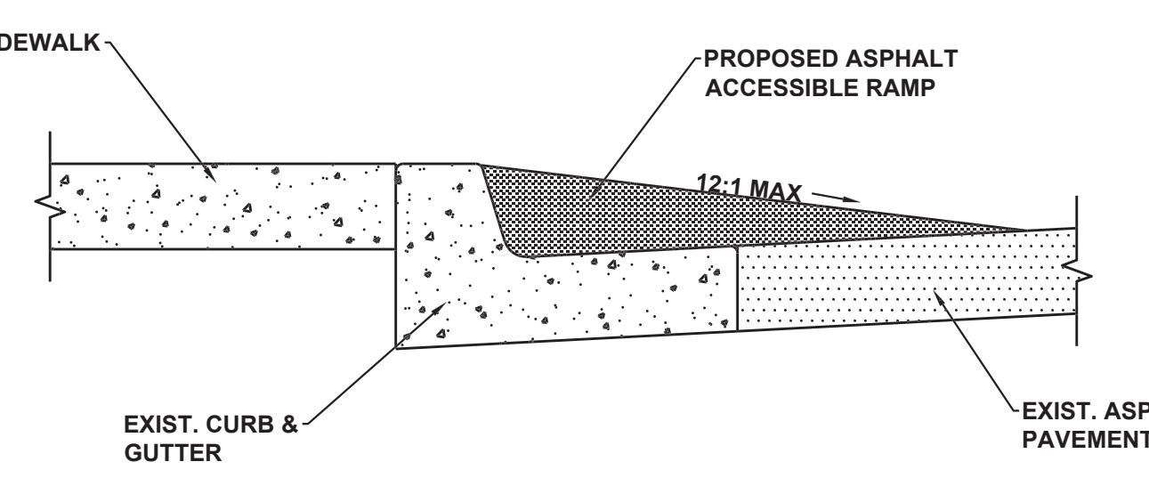
1 TEMPORARY ASPHALT ACCESSIBLE RAMP NOT TO SCALE
