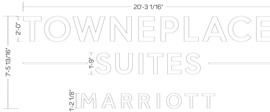
GRAPHIC DETAIL SCALE: 1/4" = 1'-0"
