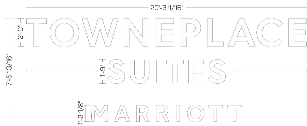
GRAPHIC DETAIL SCALE: 1/4" = 1'-0"
