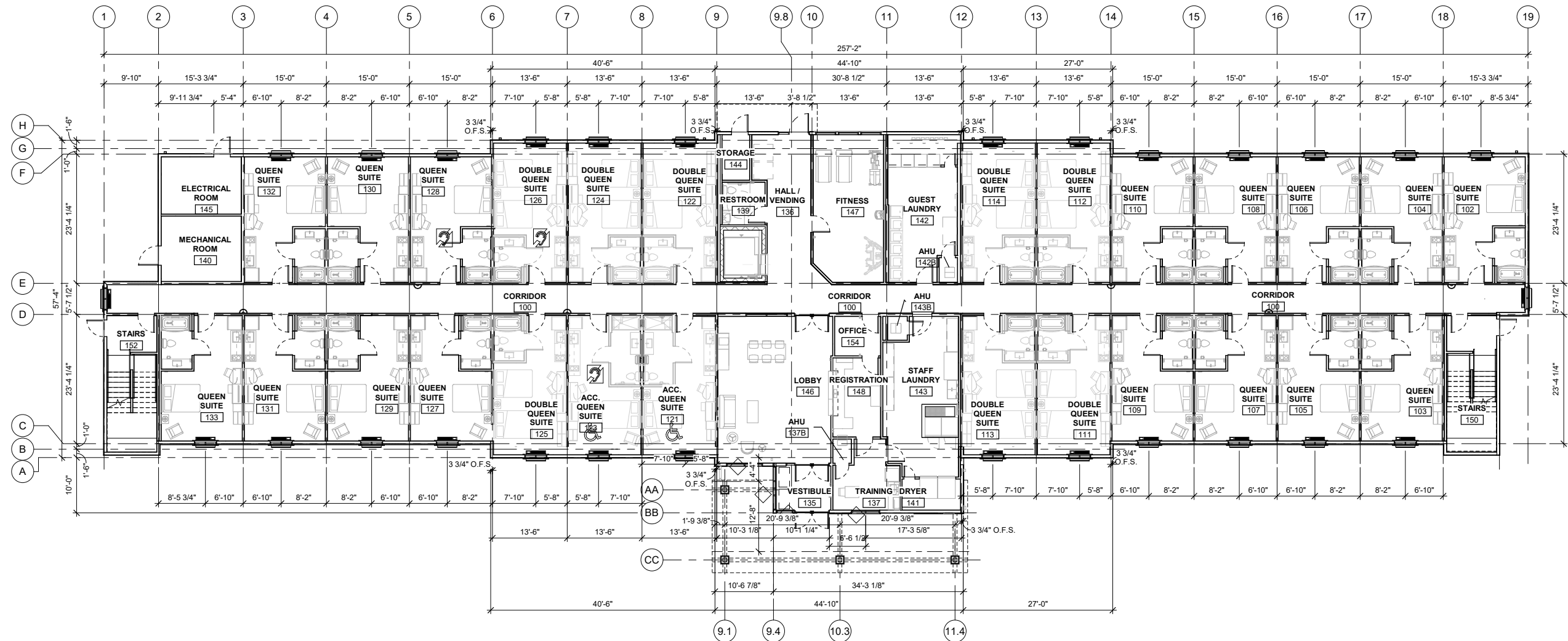
1 FIRST FLOOR PLAN NTS
