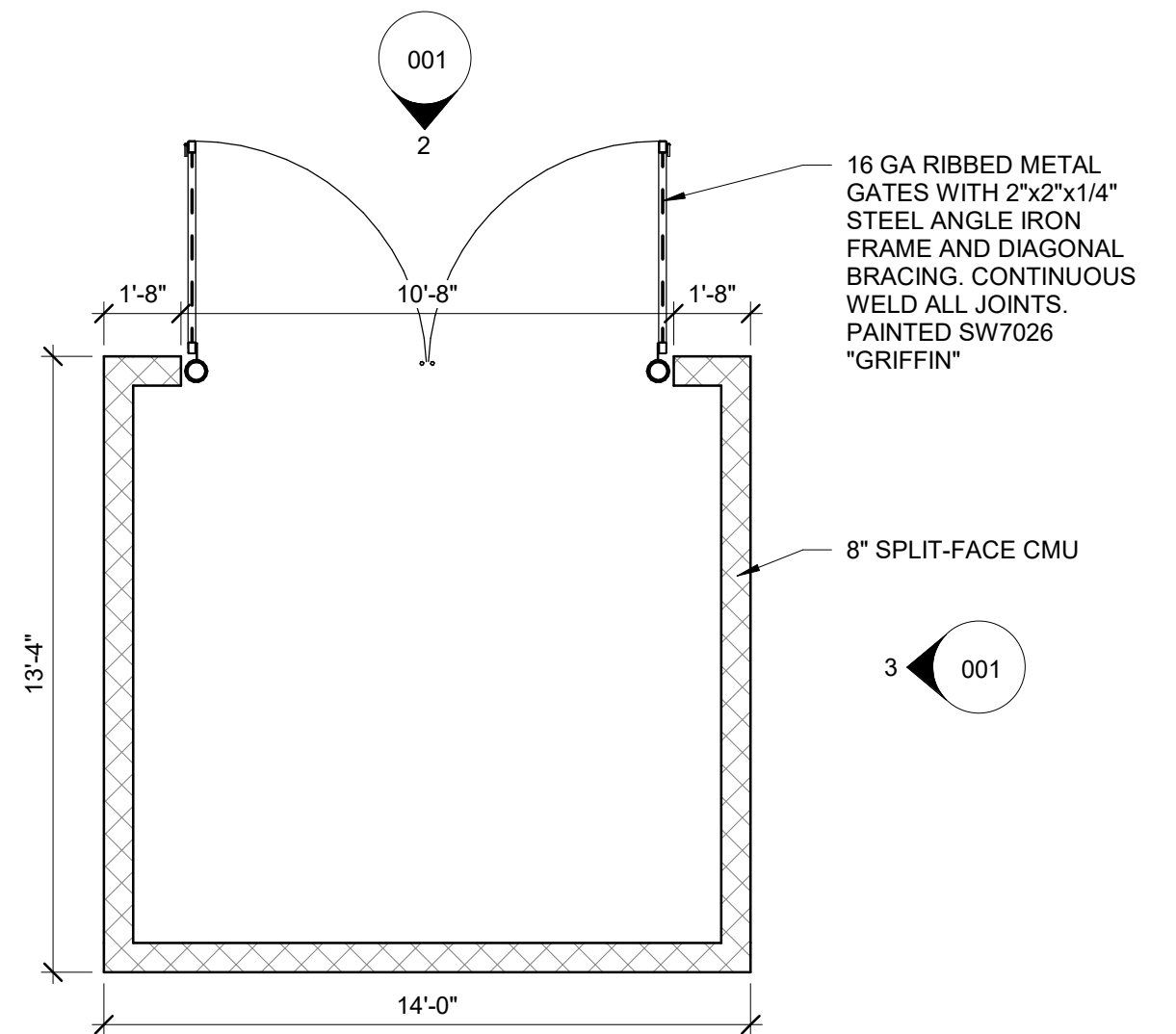
1 DUMPSTER ENCLOSURE 1/4" = 1'-0"
