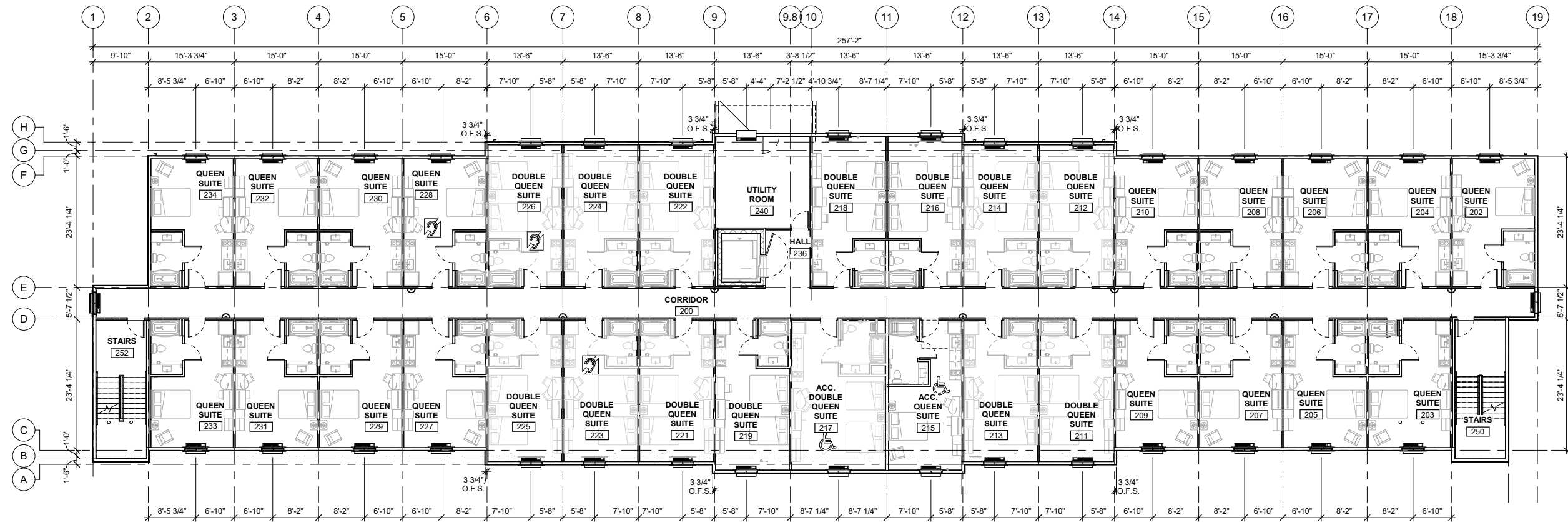
2 SECOND FLOOR PLAN NTS
