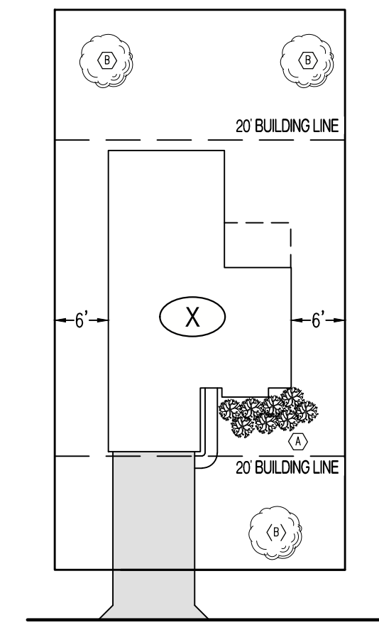
TYPICAL SINGLE FAMILY PUD LANDSCAPING
