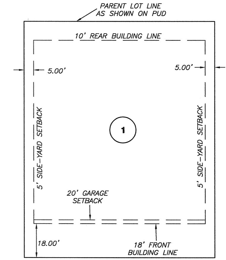
TYPICAL FUTURE ZERO LOT-LINE VERSION 1 SCALE: 1" = 30'
