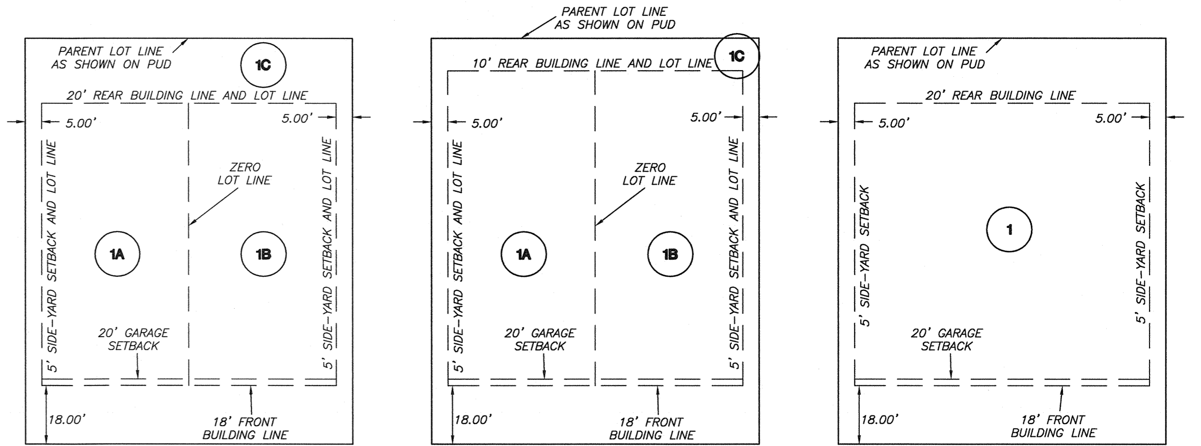
TYPICAL FUTURE ZERO LOT-LINE VERSION 1 SCALE: 1" = 30'
