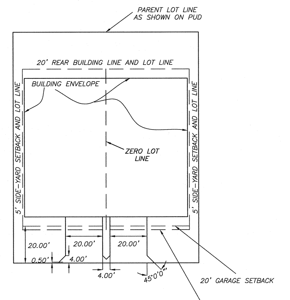
TYPICAL LOTS DRIVEWAY 2 SCALE: 1" = 30'
