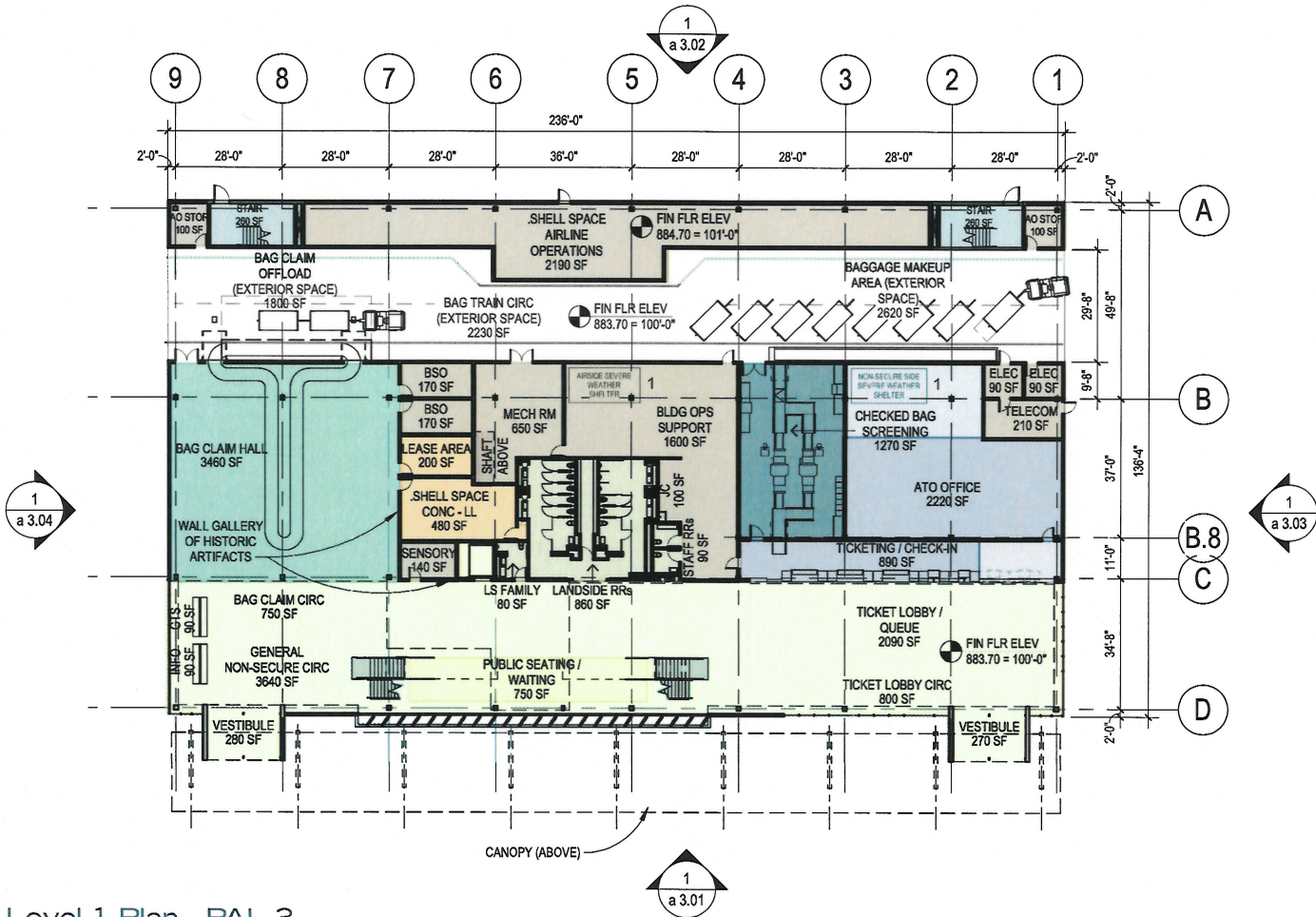
Level 1 Plan - PAL 3
