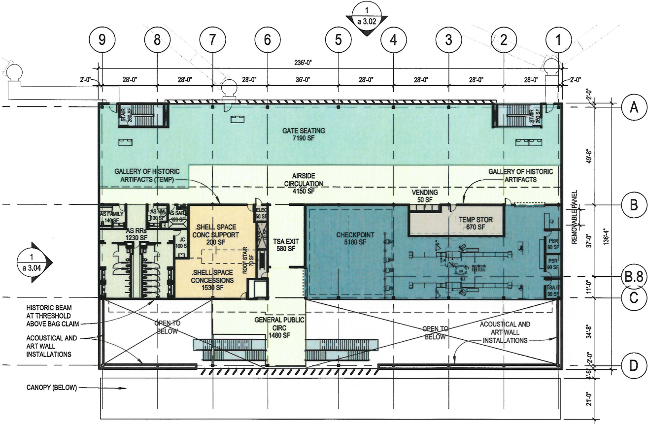
Level 2 Plan - PAL 3
