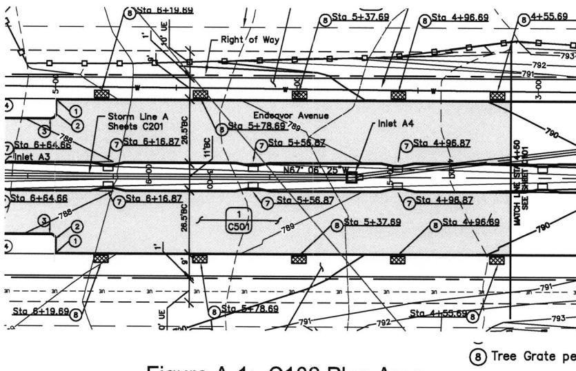
Figure A-1: C102 Plan Area
