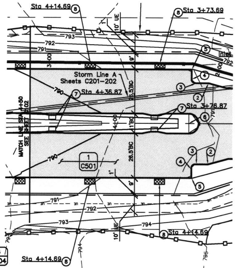
Figure A-2: C101 Plan Area
