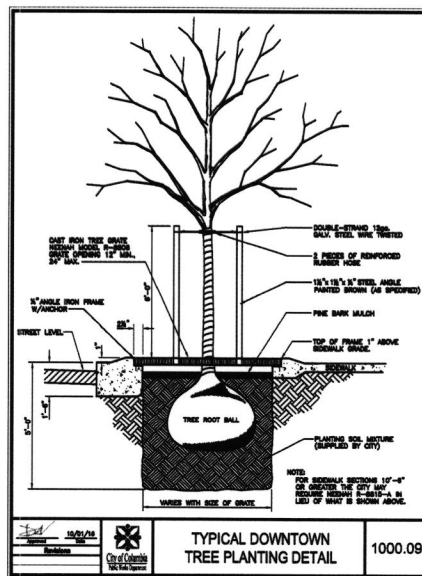
6 C504 TREE PLANTING DETAIL N.T.S.
