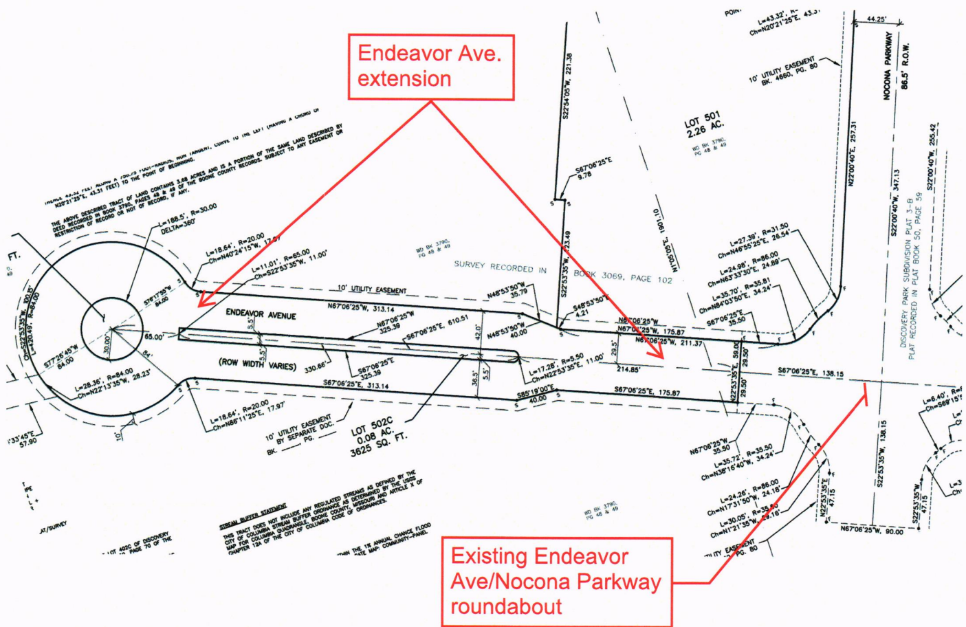
Figure B-1: Proposed Endeavor Avenue extension Right of Way
