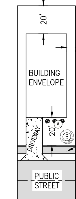
TYPICAL LOT LAYOUT REQUIRED PARKING 2 SPACES PER UNIT.
