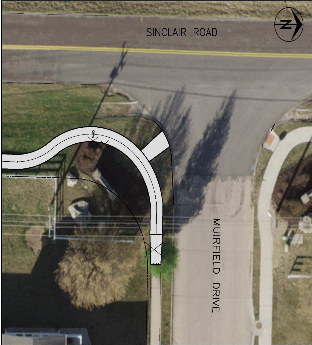
INTERSECTION OF SINCLAIR ROAD AND MUIRFIELD DRIVE
