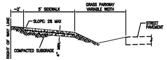
SIDEWALK WITH GRASS PARKWAY
