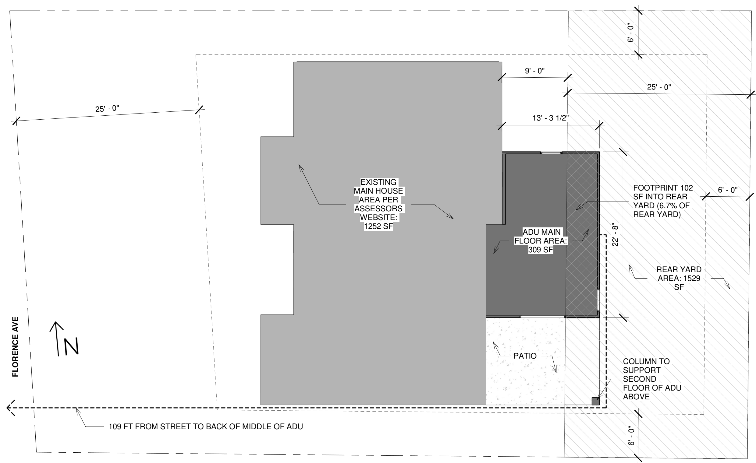
① MAIN FLOOR PLAN SITE PLAN 1/8" = 1'-0"
