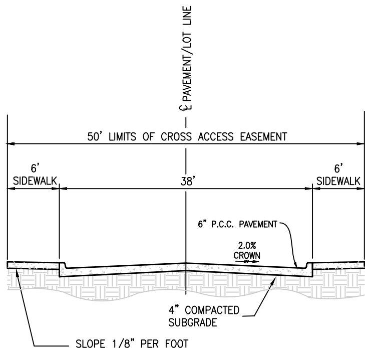
NOTE: TYPICAL CROSS SECTION OF NEW PRIVATE STREET.
