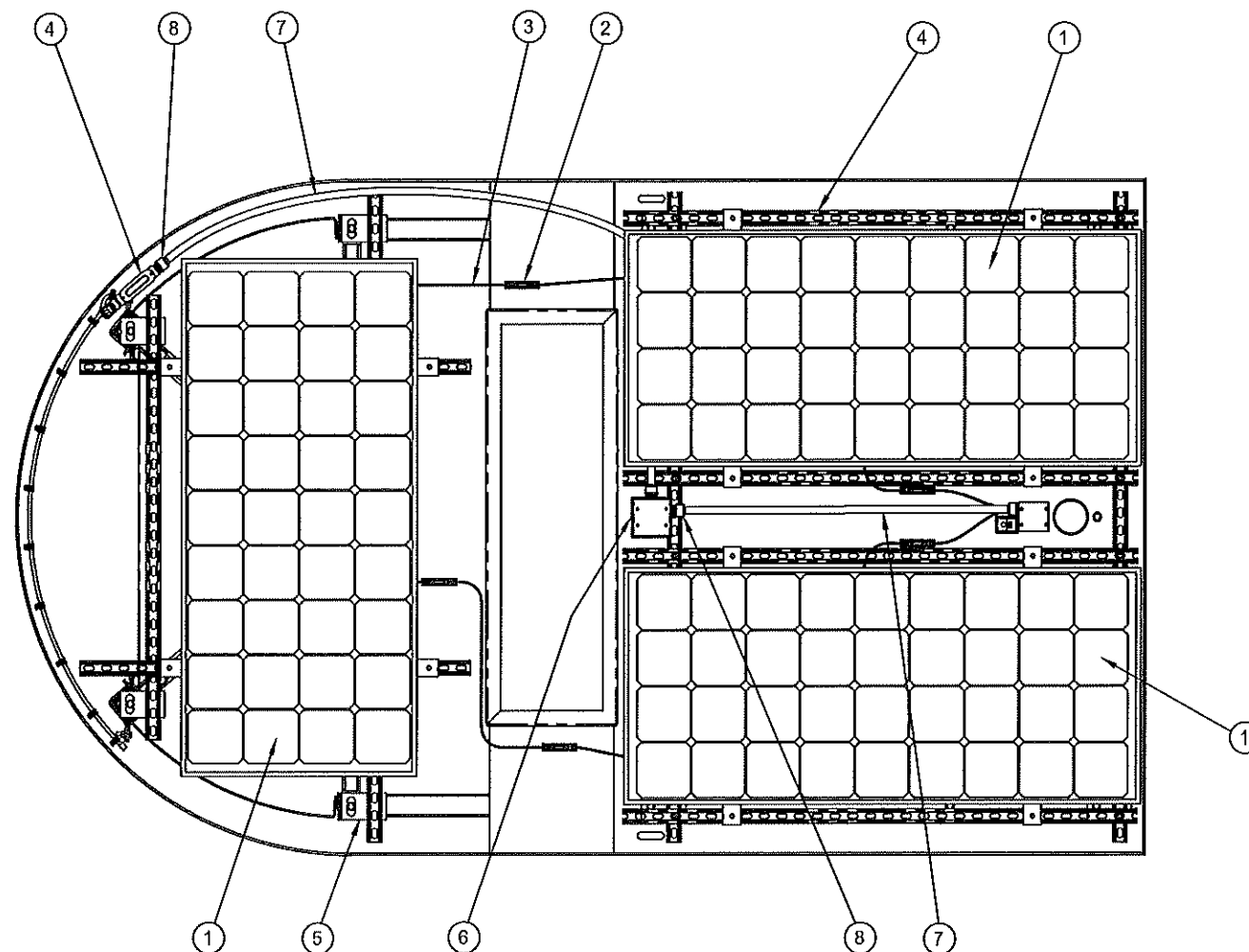
SOLAR ROOF PARTS
