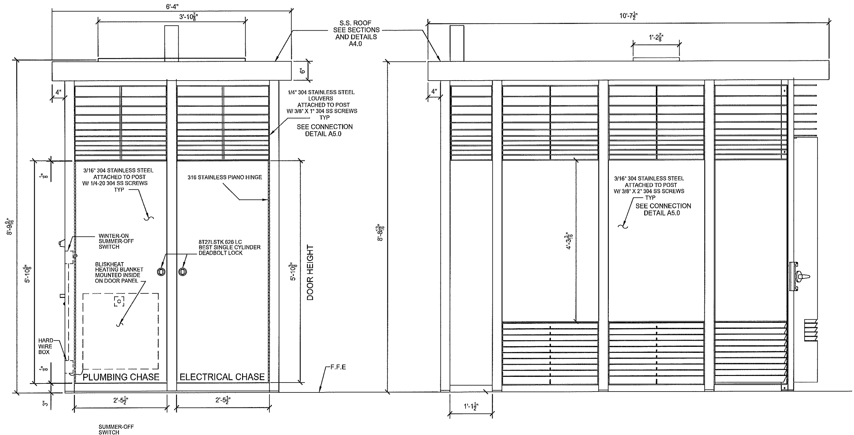
1 A3.0 BACK ELEVATION VIEW
