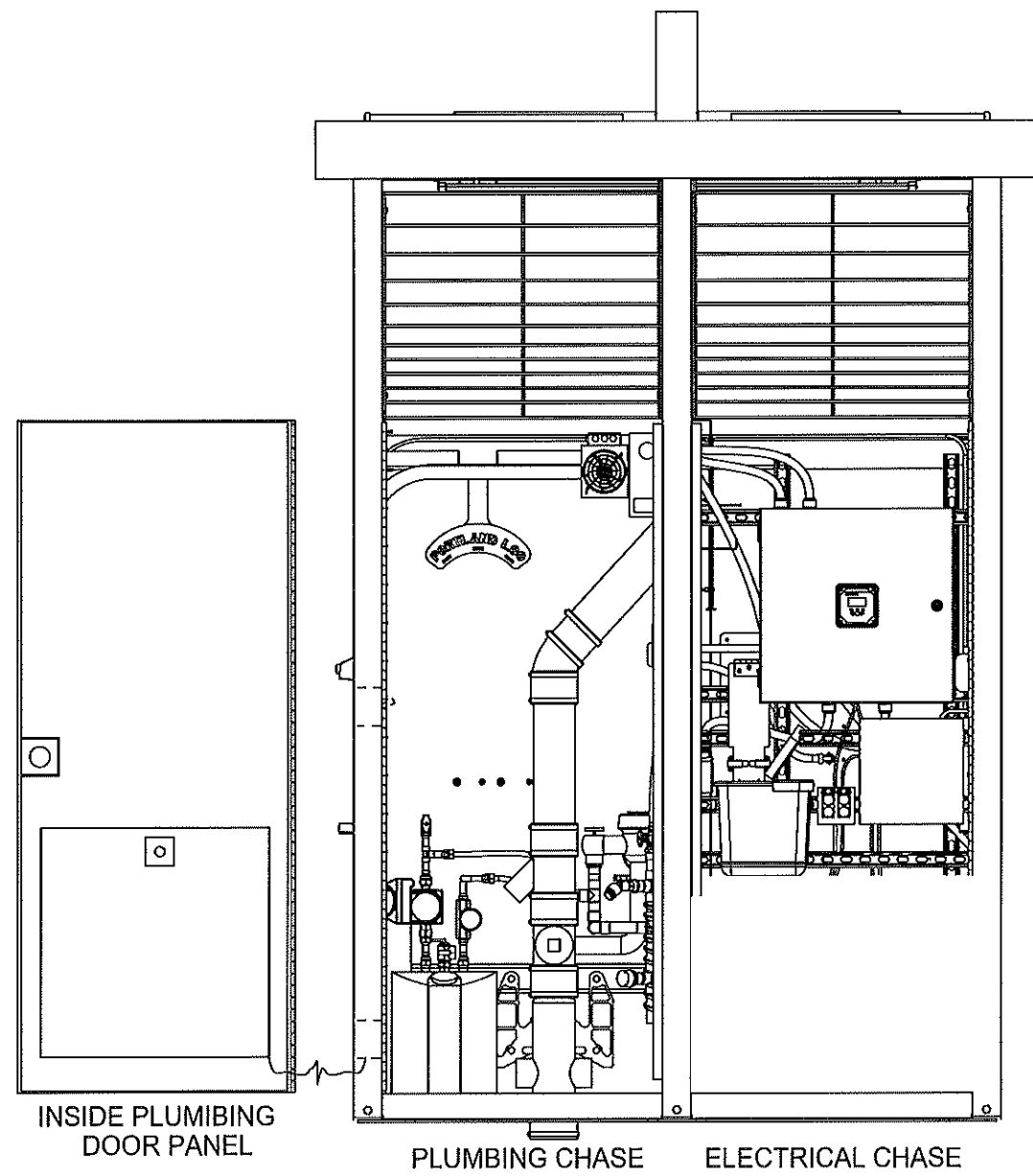
1 A3.0 BACK INTERIOR ELEVATION VIEW
