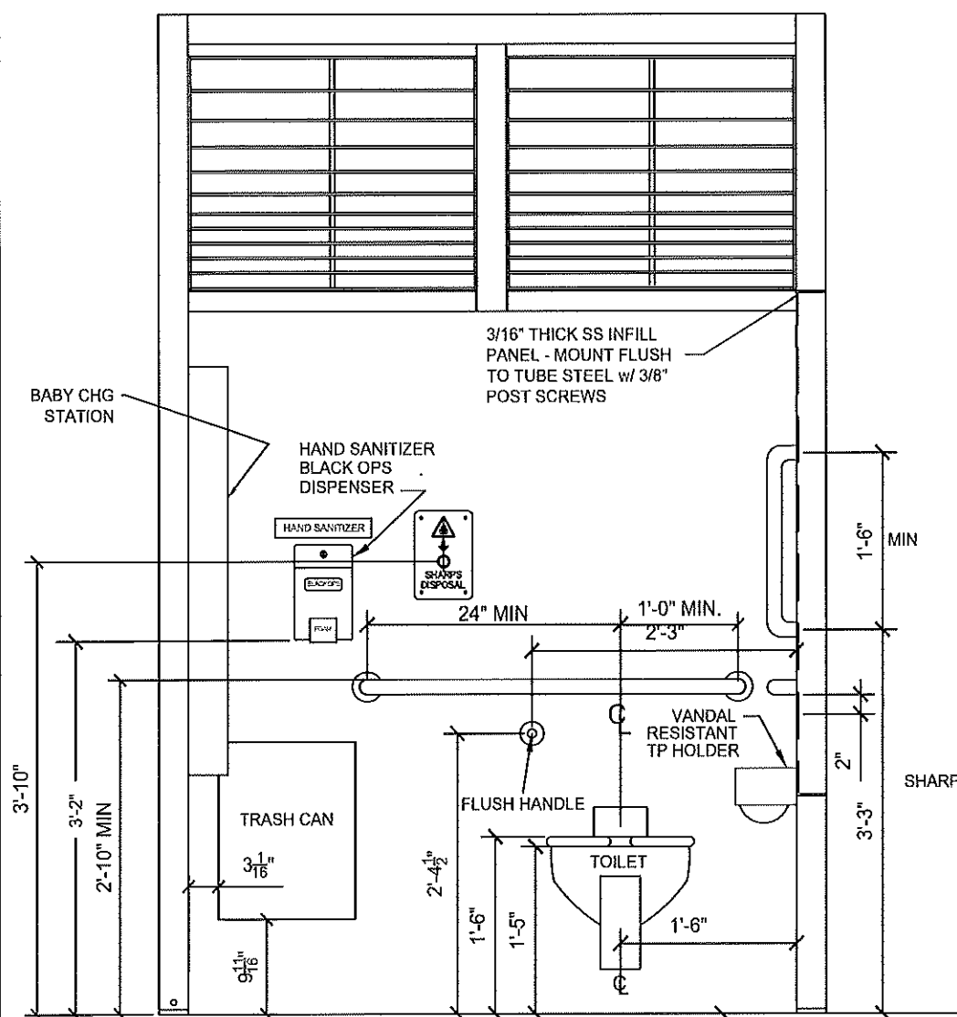
1 WATER CLOSET RAILING A6.0 1 1/2"Øx.120" wall ss PL 3/16" 304 SS (1) Assm REQ'D
