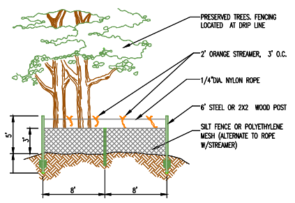
CLIMAX FOREST PROTECTION DETAIL
