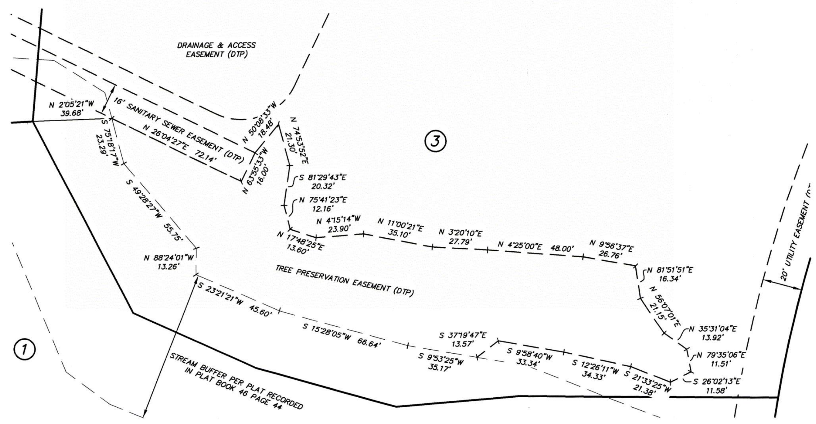
TREE PRESERVATION EASEMENT DETAIL
