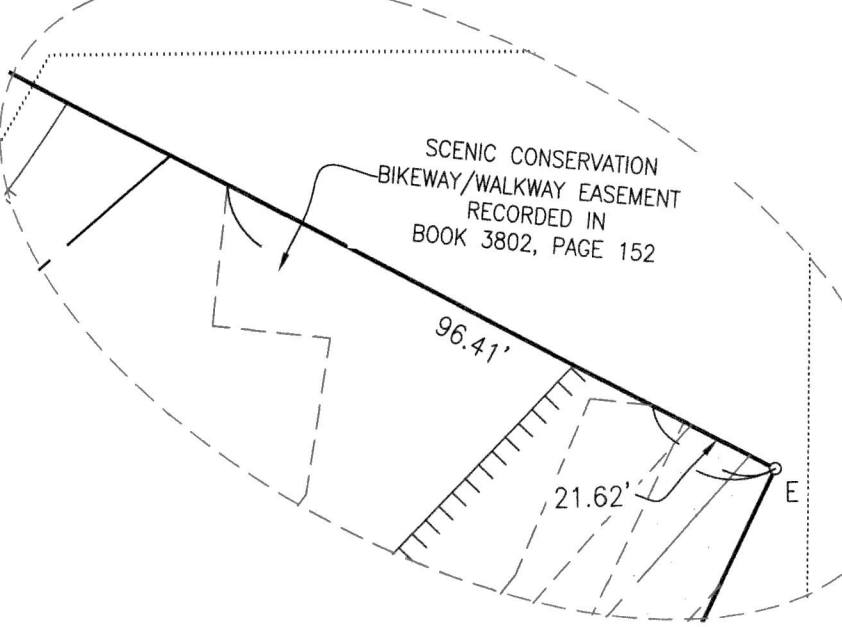
DETAIL C SCALE - 1"=30'
